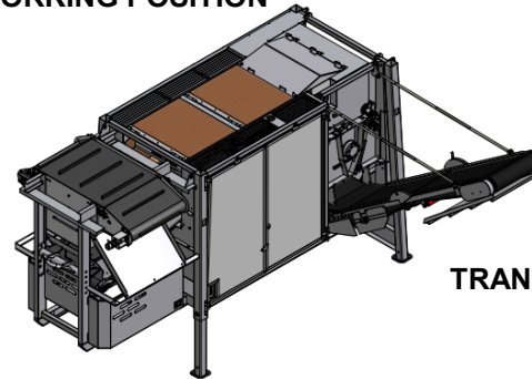
WORKING POSITION
