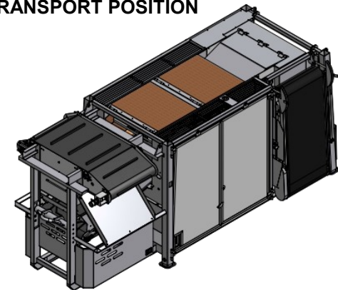
TRANSPORT POSITION
